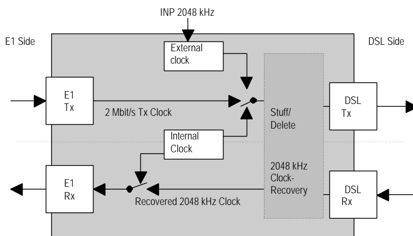
Figure 4-1: Clock Sources
