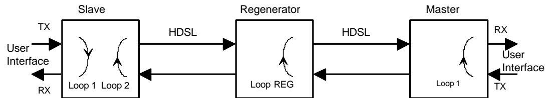
Figure 12-21: Regenerator Loopback
