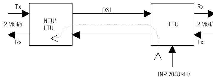
Figure 4-3: External Clock Mode
