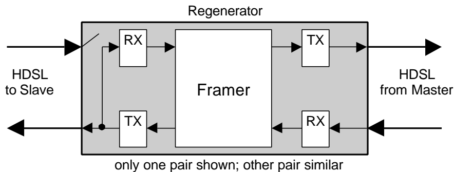
Figure 12-22: Regenerator in Loopback Mode
