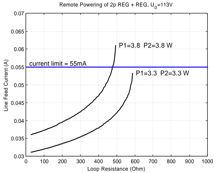
Figure 7-18: LTU powering two REGs: Line feed current vs loop resistance two different REG power consumptions
