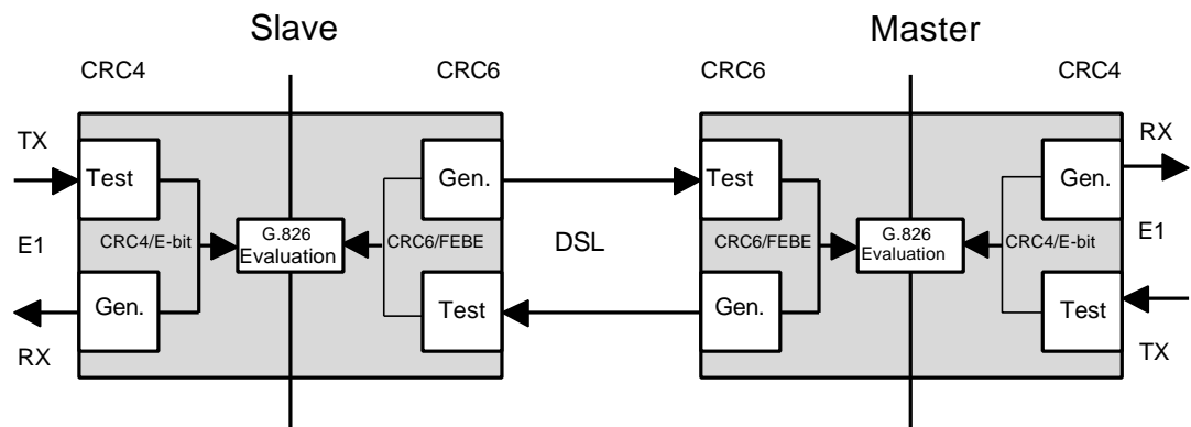
Figure 5-14: E1 G.826 Performance Evaluation
