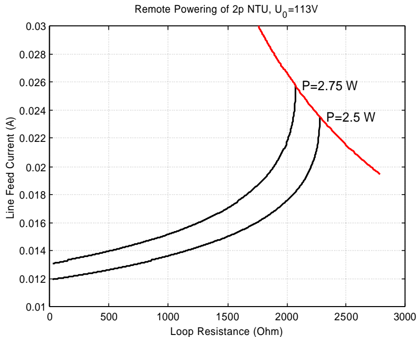
Figure 7-16: Line feed current vs loop resistance for different NTU power consumptions
