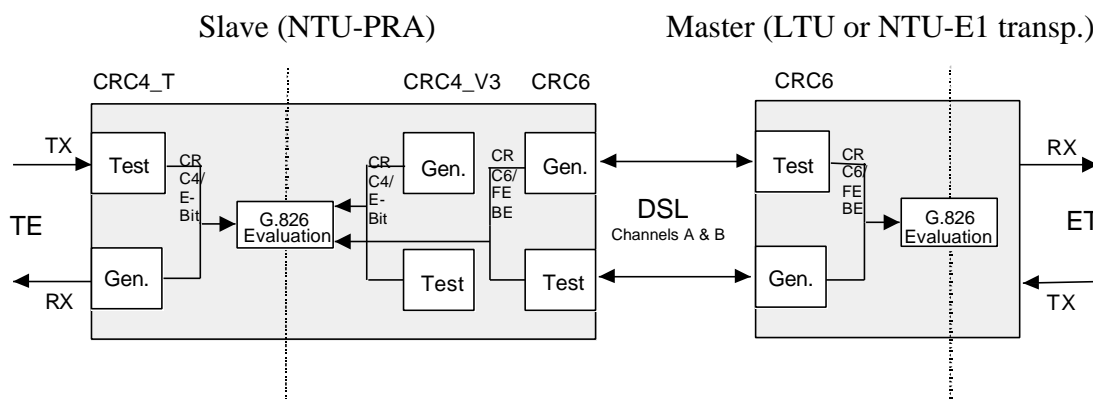
Figure 5-15: PRA G.826 Performance Evaluation
