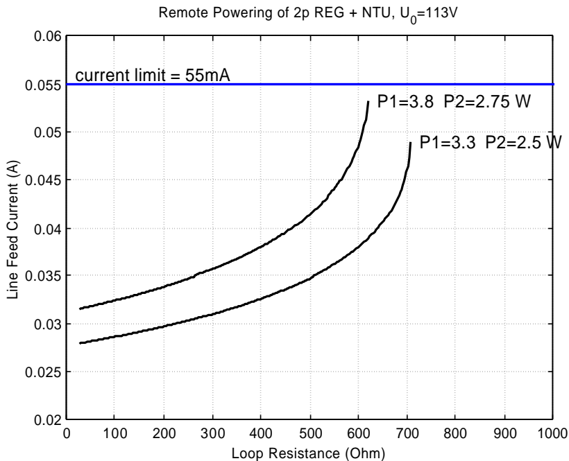
Figure 7-17: LTU powering one REG and one NTU: Line feed current vs loop resistance two different REG power consumptions
