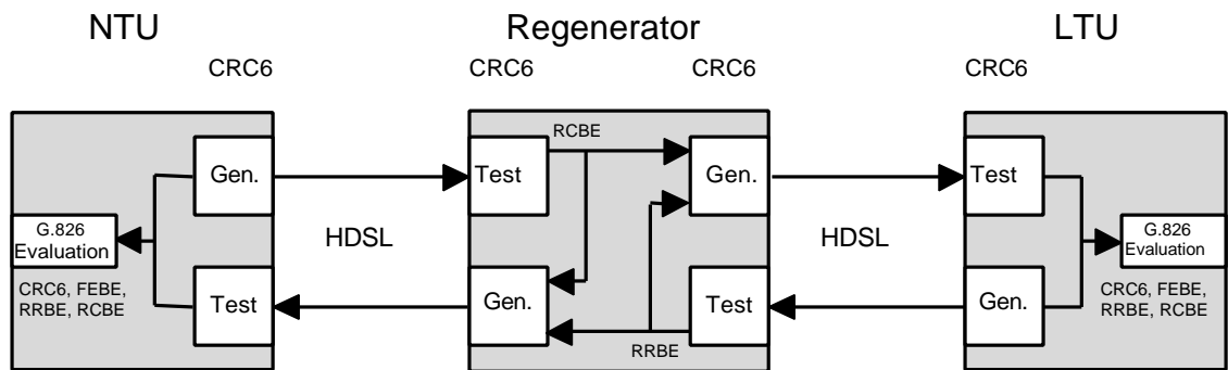
Figure 5-13: Regenerator G.826 Performance Evaluation
