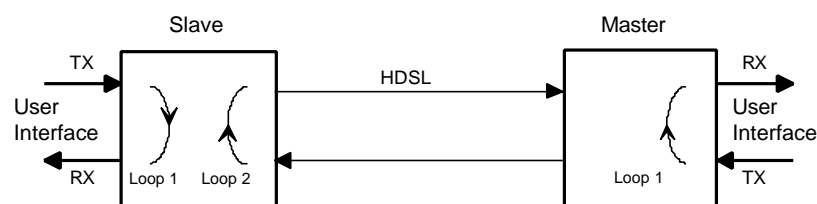
Figure 12-20: Standard Test Loops
